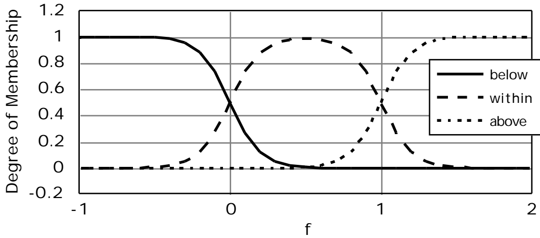
Figure 7 Short-Period Damping Requirement Membership Functions
