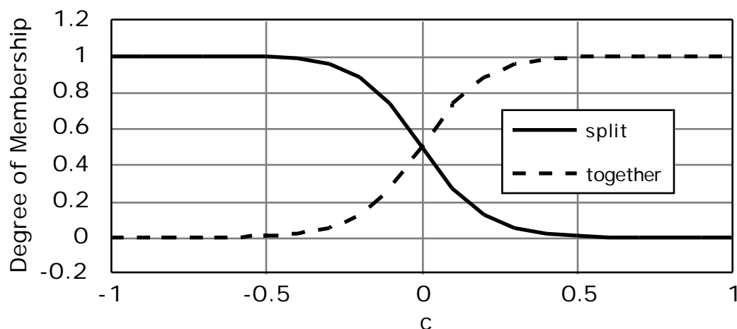
Figure 2 Short-Period Pole Grouping Membership Functions
