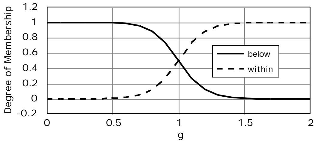
Figure 8 Short-Period Natural Frequency Requirement Membership Functions
