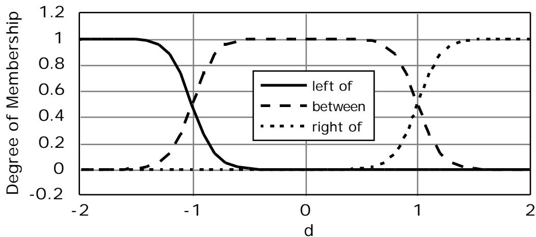
Figure 4 Short-Period Zero Location Membership Functions
