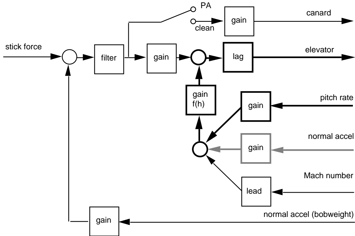
Figure 10 XB-70 Longitudinal Control System
