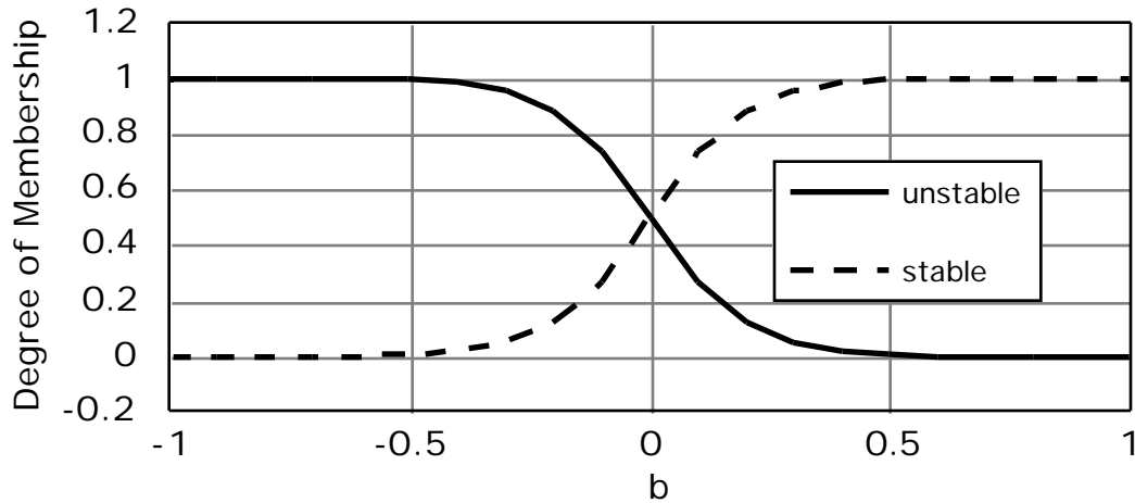
Figure 3 Short-Period Pole Stability Membership Functions
