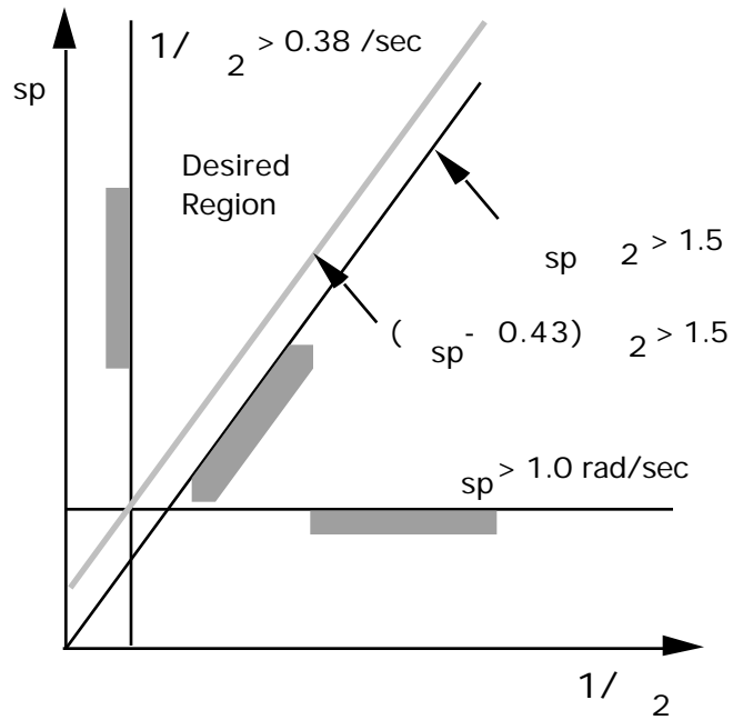
Figure 5 Short Period Design Goals
