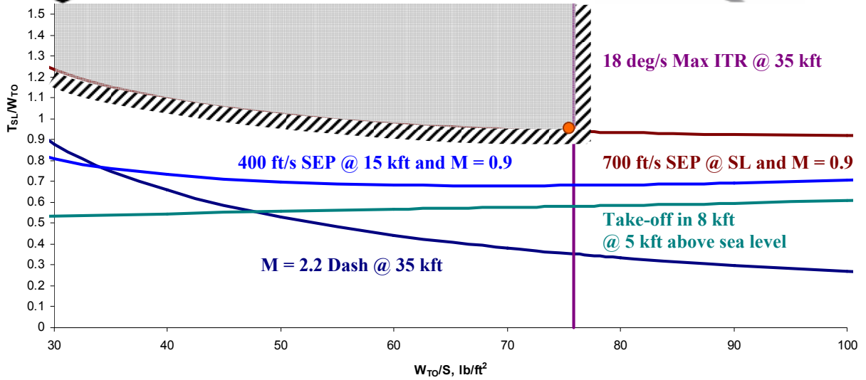
Figure 1.1: Plot of the variable sweep design's constraint curves, where the two main boundaries for the aircraft were modeled by the 18 deg/s maximum instantaneous turn rate and the 700 ft/s specific excess power curve at sea level and mach 0.9. The maximum instantaneous turn rate limited the aircraft to a wing loading at take-off of 76 psf.
