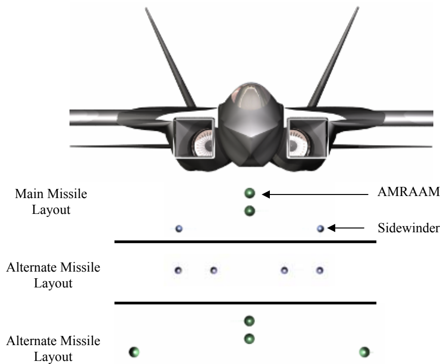
Figure 8.46: Various Missile Loading Configurations
