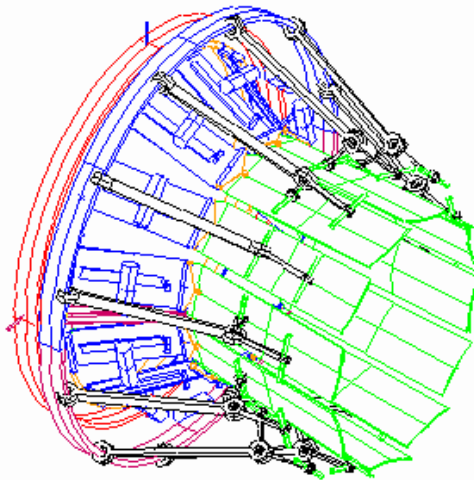
Figure 5.24: Thrust vectoring convergent-divergent nozzle for the Shrike interceptor.
