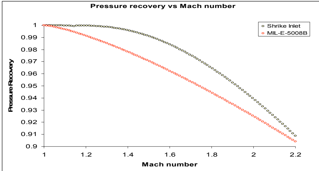
Figure 5.23: Shrike inlet pressure recovery vs. military requirements
