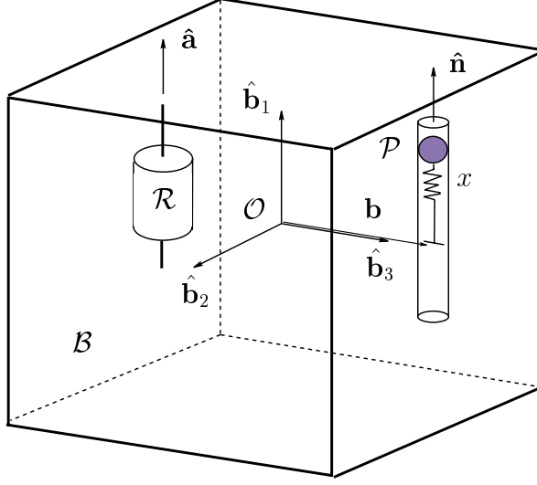
Figure 1: Single-rotor axial gyrostat with aligned discrete damper
